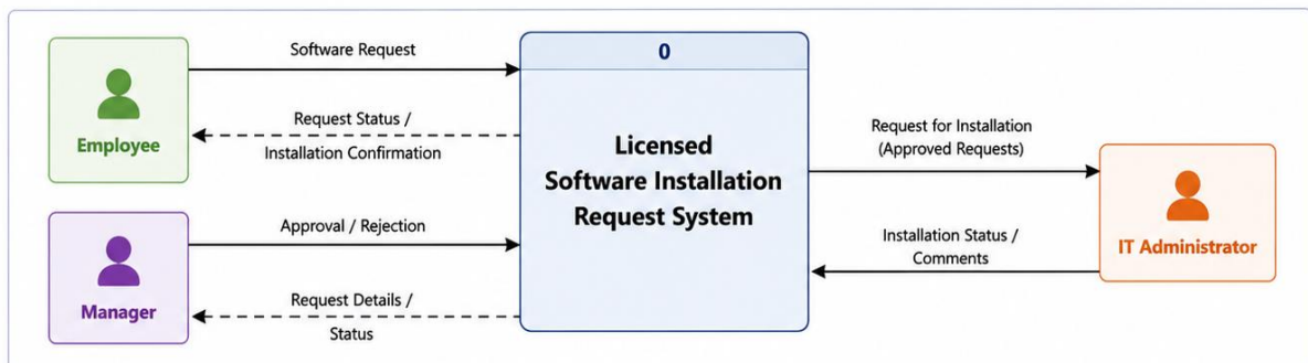
Figure 1: DFD – Level 0 (Context Diagram)
