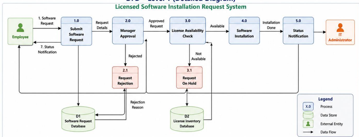
Figure 2: DFD – Level 1 (Detailed Diagram) with Example
